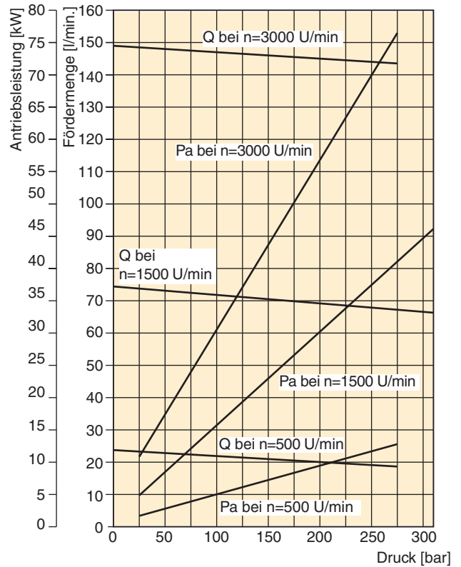
PGP640 - 50,0 cm 3
