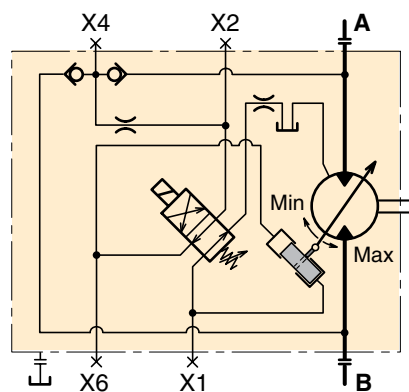
EO H 01 I-Schaltplan (Magnetspule stromlos).
